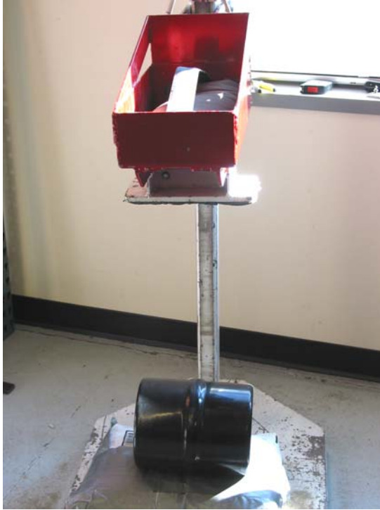
Figure 2. No-Fed-Bear Canister on MTDC Impact Test Stand
